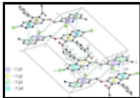
Fig. 2. \pi - \pi interactions (dotted lines) in the crystal structure of the title compound. Cg denotes the ring centroids. [Symmetry codes: (i) -x, -y + 1, -z + 2 ; (ii) -x + 1, -y + 1, -z + 1 ; (iii) x + 1, y, z - 1 .]
